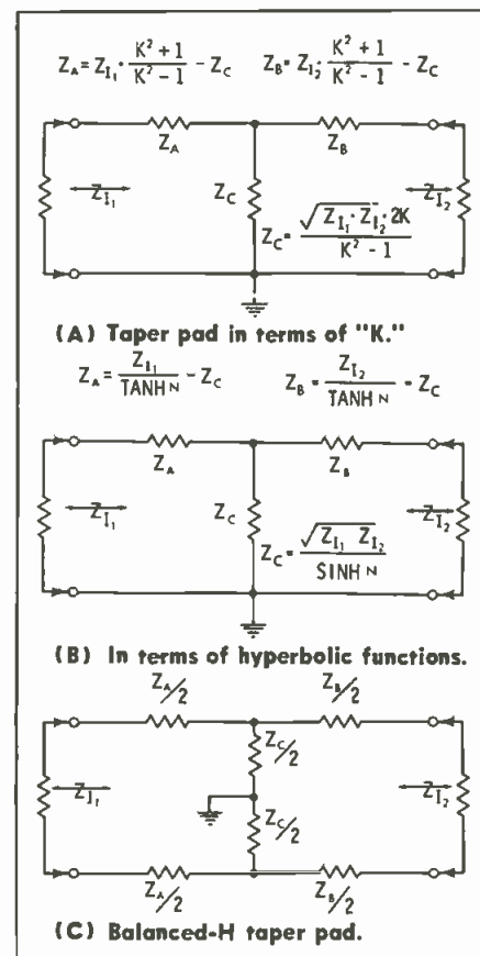
Fig. 5. Two dissymmetrical taper networks.
