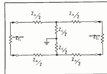
Fig. 3. A symmetrical balanced-H pad.
