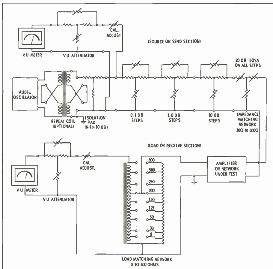
Fig. 6. Unbalanced transmission set employing rotary impedance matching network.
