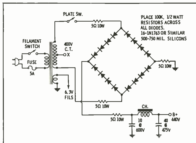
Fig. 1(B). Bridge power supply for converted remote transmitter.
