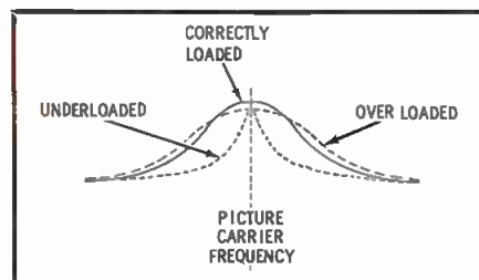
Fig. 4. Curves for three amplifier loads.
