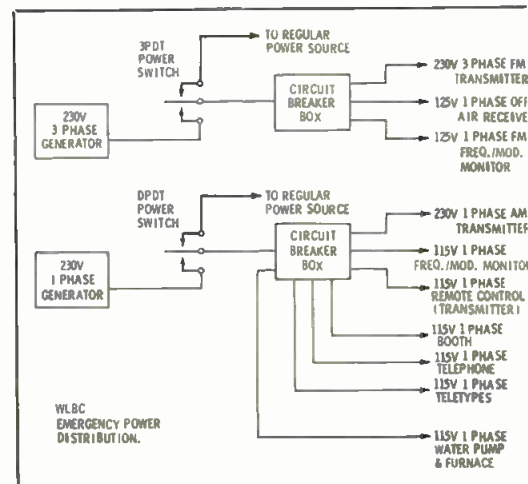
Fig. 5. Diagram of power routing system.
