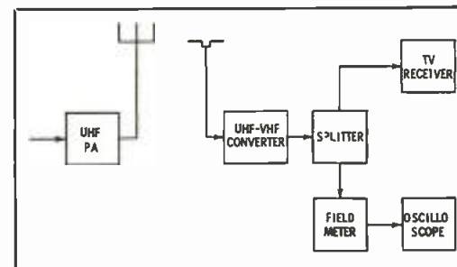
Fig. 2. Test setup for test point three.
