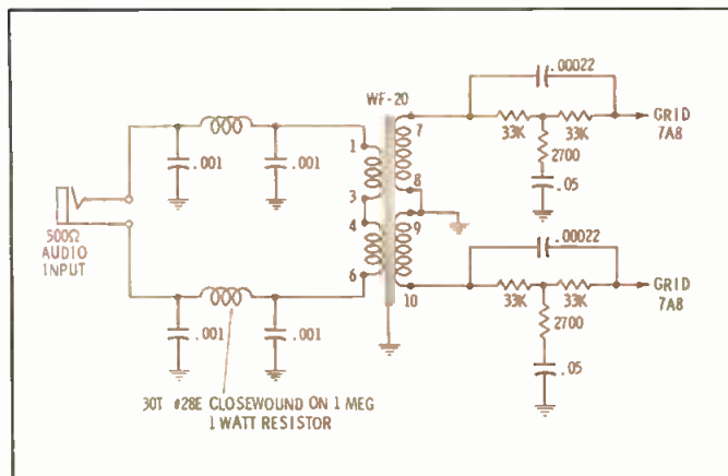
Fig. 3. Audio input equalizing network to correct response.
