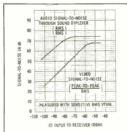
Fig. 2. Graph of STL microwave s/n ratio.
