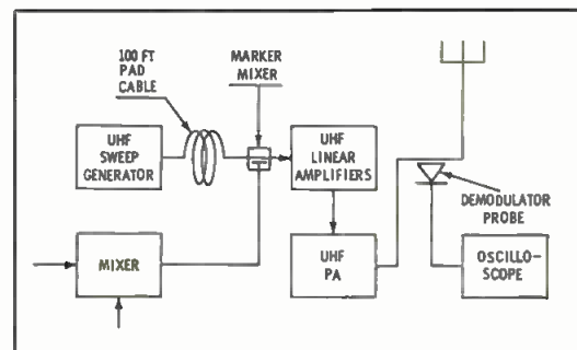
Fig. 3. The test setup for section three.
