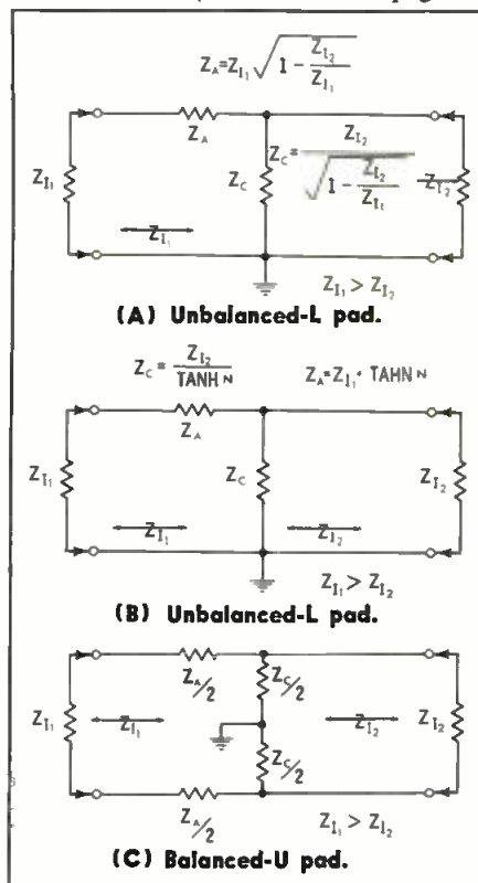
Fig. 7. Minimum-loss resistance networks.
