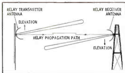
Fig. 7. Beams above and below path. the line of the signal path properly illuminates the flat surface to produce the predicted gain and signal-to-noise ratio. An increase in signal strength of a few db may be obtained by judiciously adjusting the reflector curvature. When the reflector surfaces have been properly aligned, the driving antenna should be moved in both azimuth and elevation to establish the proper maximum signal at the STL receiver site. Fig. 8 illustrates a passive reflector and antenna illustration.
